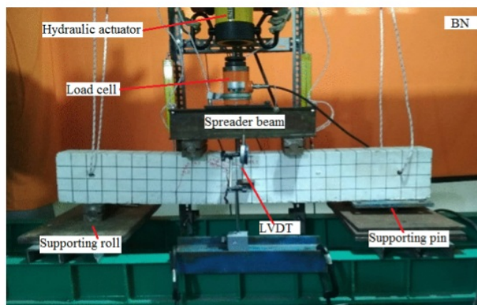
Figure 3. Flexural testing on RC beam BN model.
