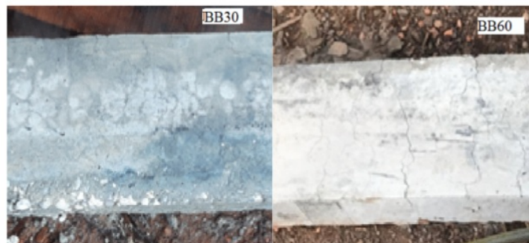
Figure 8. Discolouration of the post-fire RC beams after 30 and 60 minutes.
