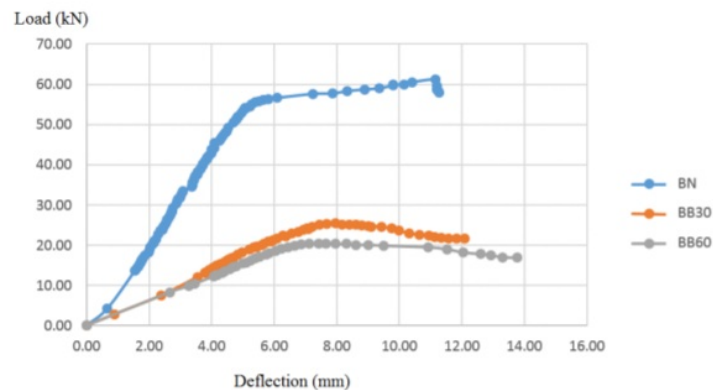
Figure 7. Relationship curves of deflection and loads.
