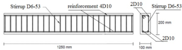
14 Figure 1. Detail of reinforced concrete beam.
