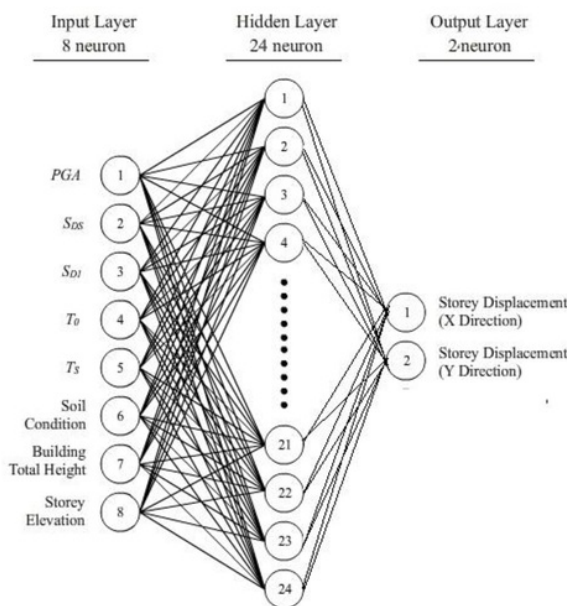
Fig.3. Proposed Backpropagation (BPNN) Architecture
