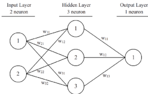
Fig.1. Simple Artificial Neural Network Scheme
